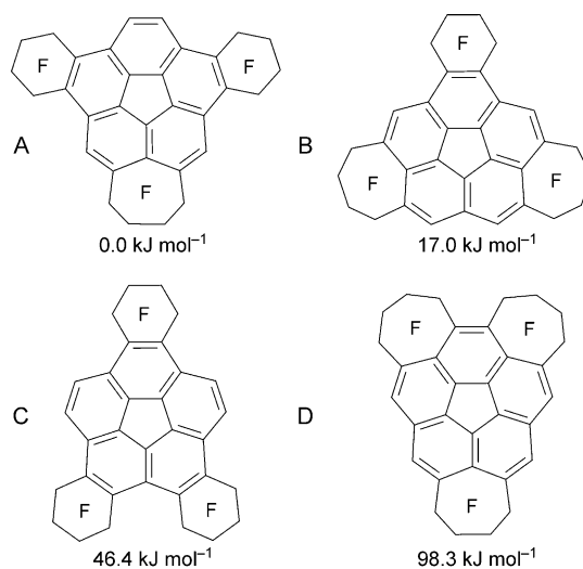
Figure 3. Structures and DFT-calculated relative energies of four possible C_s\text{-}C_{20}H_4(C_4F_8)_3 molecules.
