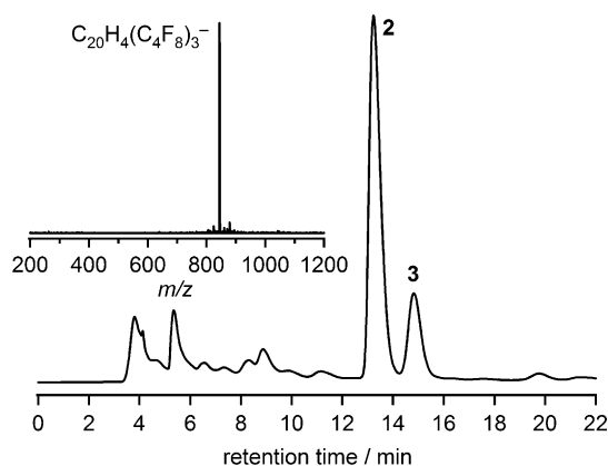
Figure 1. HPLC trace of the crude product formed in the reaction of corannulene with 1,4\text{-}C_4F_8I_2 (Cosmosil Buckyprep column, 20:80 v/v toluene/ n -heptane eluent at a flow rate of 5\text{ mL min}^{-1} ; 300 nm detection wavelength). Inset: NI-APCI mass spectrum of purified 2 (the mass spectrum of 3 is very similar).
